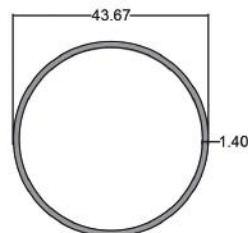
لوله Tube code: PN00017 3.200 kg
