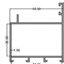
لنگه Vent Profile code: PNP6002 6.500 kg
