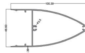
دوک Grap Profile code: CWS006 6.400kg
