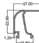
زهوار گرد تک جداره Round Rickety (Single Walled) code: PM00014 1.800 kg
