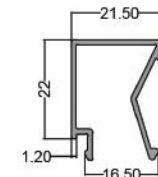
زهوار تک جداره Rickety ( Single Walled ) code: PNH0011 2.100 kg
