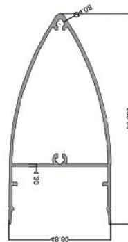
دوک Grap Profile code: CWS006 6.400 kg
