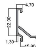
زهوار سه جداره Rickety (Triple Walled) code: PM00013 1.300 kg
