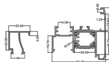
زهوار دوجداره Rickety (Double Walled) code: PLH0006 1.700 kg
