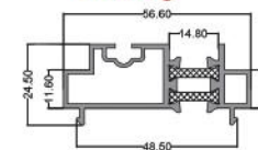
آداپتور Adapter code: PLS0006 5.00 kg
