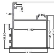
سپری Tripetalous code: K336-7 5.200kg
